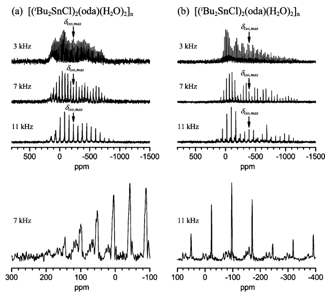
Figure 6. ^{119}\text{Sn} CPMAS NMR spectra of (a) [(\text{Bu}_2\text{SnCl})_2(\text{oda})(\text{H}_2\text{O})_2]_n ( 5 ) and (b) [(\text{Bu}_2\text{SnCl})_2(\text{oda})(\text{H}_2\text{O})_2]_n ( 6 ) acquired at MAS frequencies of 3, 7, and 11 kHz. The expansions of the MAS spectra acquired at 7 kHz (for 5 ) and 11 kHz (for 6 ) show the existence of a second Sn(IV) site which is influenced by ^1J(^{119}\text{Sn}, ^{35/37}\text{Cl}) coupling.
