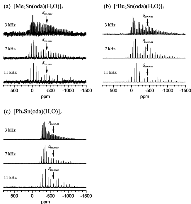
Figure 5. The ^{119}\text{Sn} CPMAS NMR spectra of (a) [\text{Me}_2\text{Sn}(\text{oda})(\text{H}_2\text{O})]_2 ( 1 ), (b) [\text{n-Bu}_2\text{Sn}(\text{oda})(\text{H}_2\text{O})]_2 ( 2 ), and (c) [\text{Ph}_2\text{Sn}(\text{oda})(\text{H}_2\text{O})]_2 ( 3 ) acquired at MAS frequencies of 3, 7, and 11 kHz.
