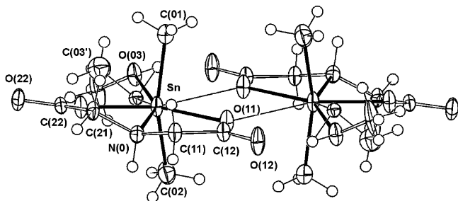
Figure 4. Centrosymmetric mutual approach of the pair of molecules of 7 . Note the disordered minor component of the methanol molecule. Sn–C(01), O(3,03'), N(1): 2.107(4), 2.109(4), 2.391(4), 2.35(1), 2.346(2), 2.156(2), 2.282(2) Å. C(01)–Sn–C(02): 159.5(1)°.
