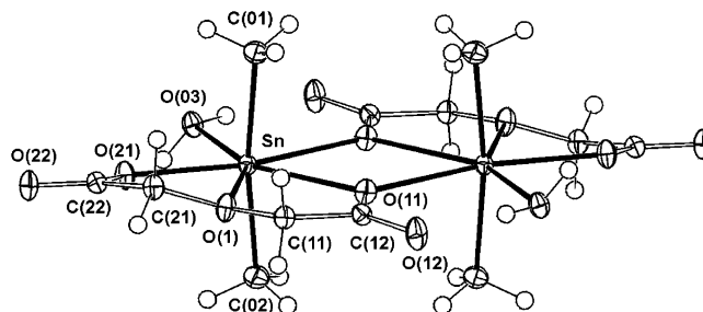
Figure 2. Single centrosymmetric dimer of 1 : Sn—C(01,02), O(03,1,11, 21,11'), 2.103(2), 2.104(2), 2.218(1), 2.357(2), 2.498(2), 2.200(2), 2.505(2) Å; O(11)⋯O(11'), 2.771(2); Sn⋯Sn', 4.1653(4) Å; C(01)—Sn—C(02), 171.59(7)°.
